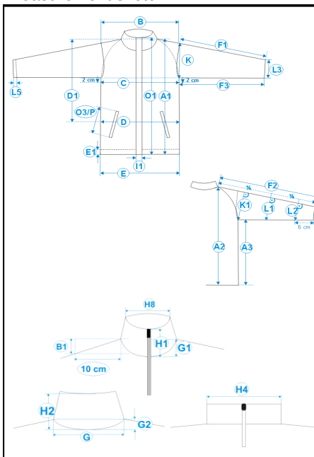
Measurement sketch
